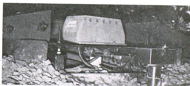
The PRR's angle iron foundation. Long bolts allow for track raise.
