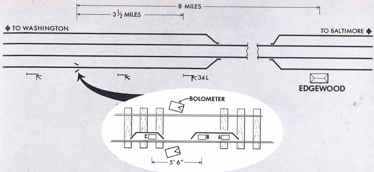
The location of the PRR's latest hot box detector installation. Four track main line reduces to two to bridge river.
